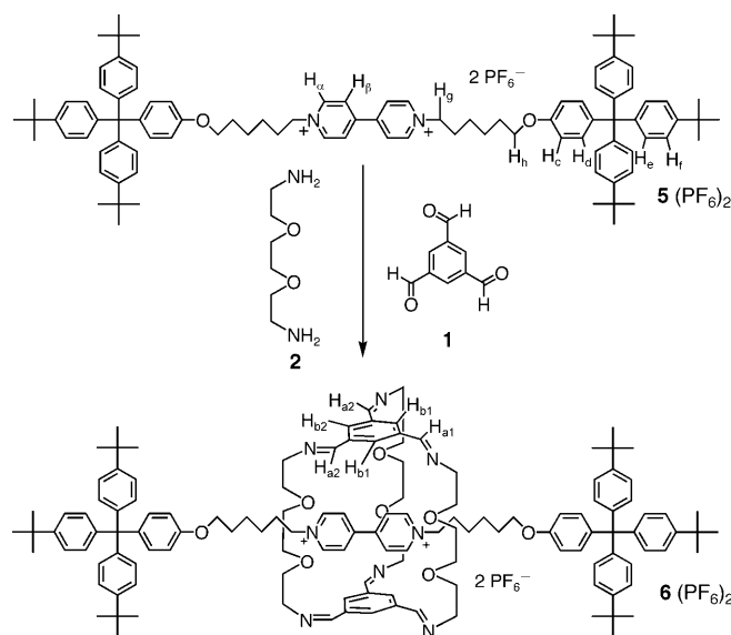
Scheme 2. Templated formation of [2]rotaxane 6 (PF 6 ) 2 .
