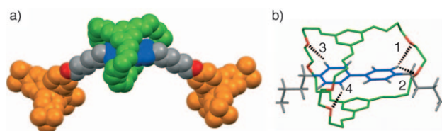
Figure 5. a) Space-filling representation of computed lowest energy co-conformation of 6 ( \text{PF}_6 ) _2 . b) Multiple \text{C}-\text{H}\cdots\text{O} hydrogen bonding interactions indicated by the stick model. Hydrogen-bonding distances \text{C}\cdots\text{O} , \text{H}\cdots\text{O} [Å] and angles \text{C}-\text{H}\cdots\text{O} [°]: 1) 3.49, 2.61, 138.6; 2) 3.45, 2.87, 147.5; 3) 3.59, 2.59, 154.1; 4) 3.47, 2.64, 133.6.
